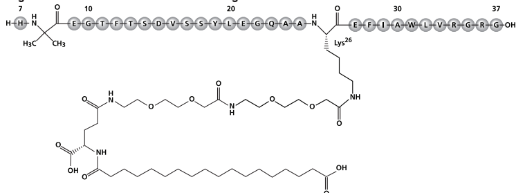
Figure 1. Structural Formula of Semaglutide
